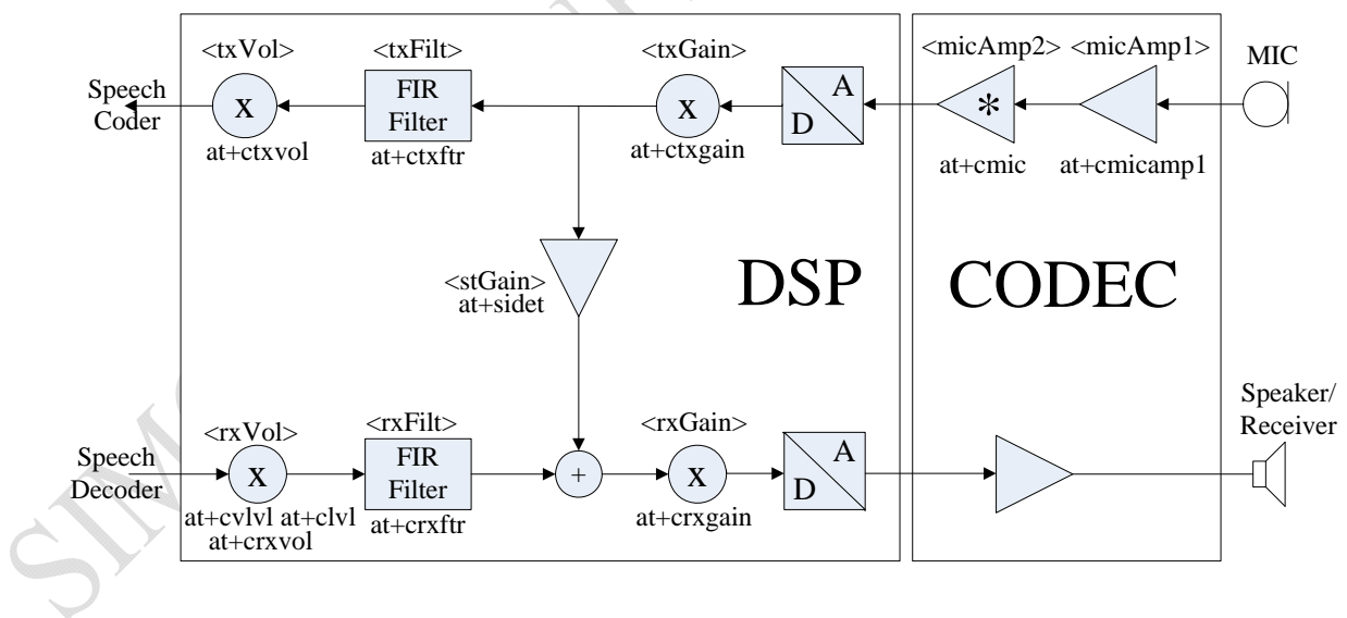
Figure 6: Audio programming model
