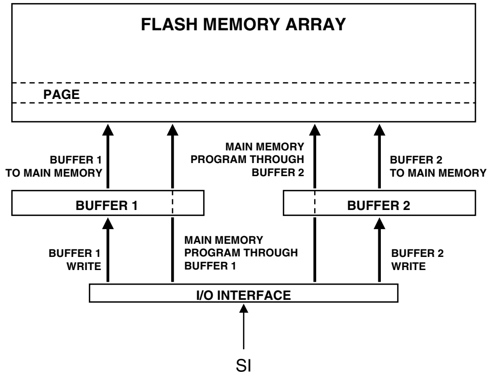
Figure 7. Serial DataFlash Write Operations
