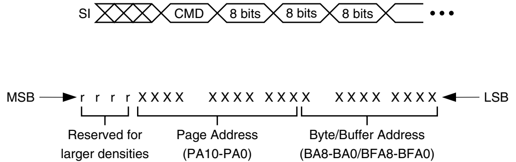
Figure 4. Command Sequence for AT45DB041B Read/Write Operations (Except Status Register Read)
