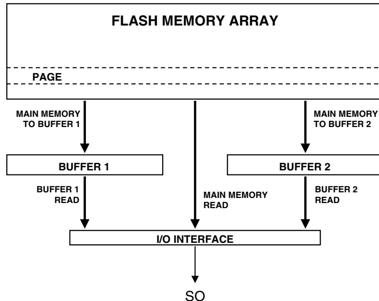
Figure 5. Data Can be Read Directly from Main Memory or Through the Buffers
