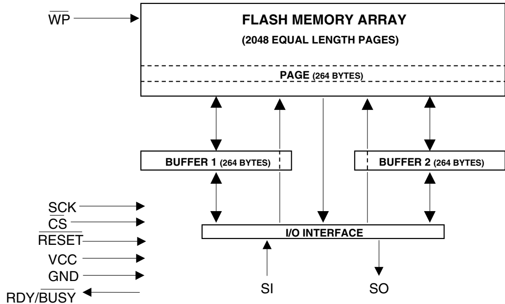
Figure 1. Atmel's AT45DB041B Serial DataFlash Consists of a Flash Memory Array, Two Buffers and a Simple I/O Interface
