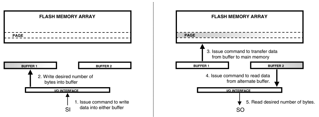
Figure 6. Serial DataFlash Supports Virtual Read-while-write Operations
